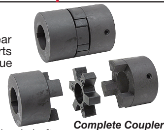
Complete Coupler
