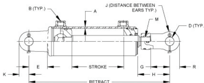
Dimensional Data
