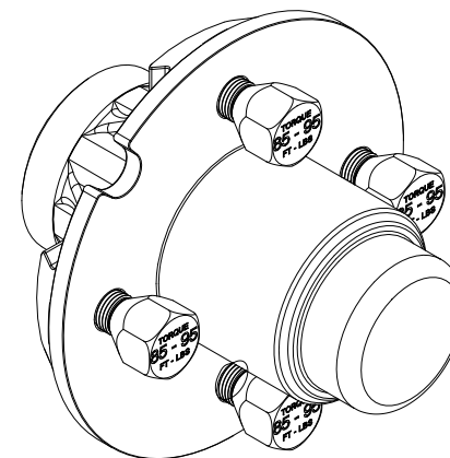
OUTBOARD VIEW
