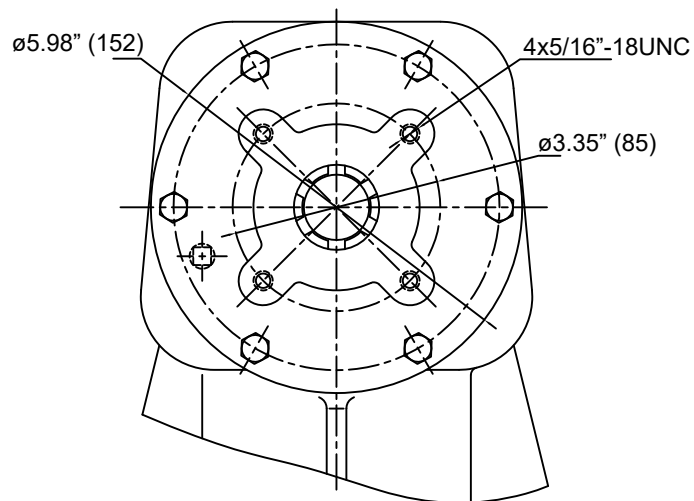
VIEW K
