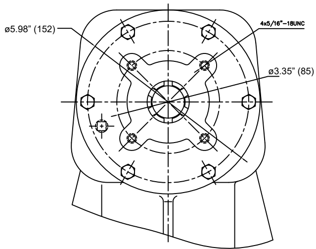
VIEW K
