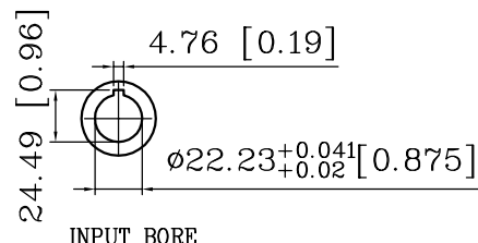
INPUT BORE
