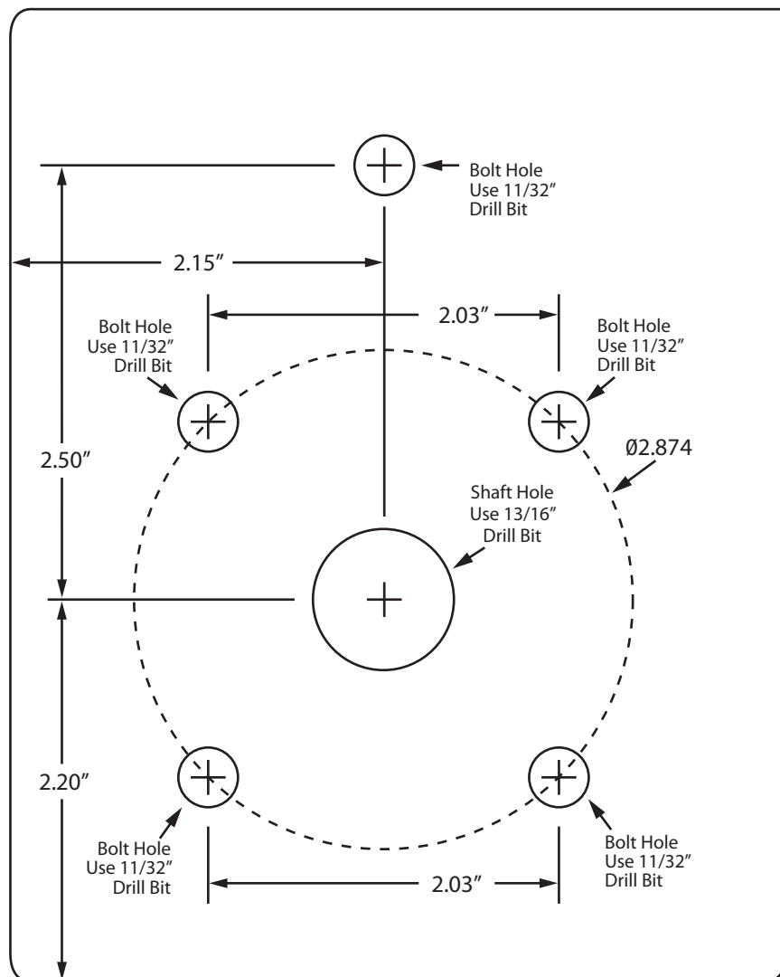
Gearbox
