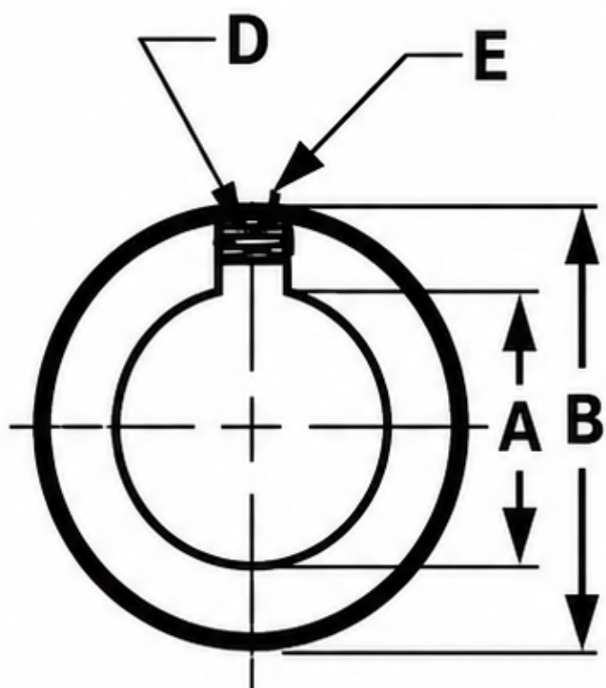
Round Bore
