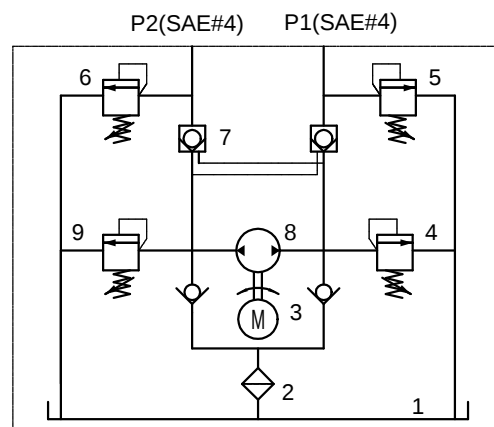
Hydraulic Schematic
