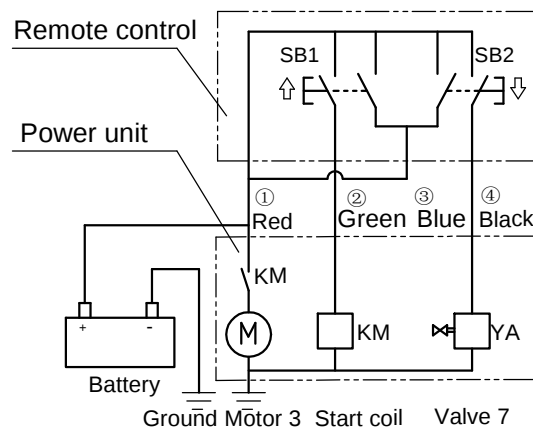
ELECTRICAL SCHEMATIC
