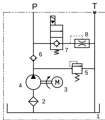
HYDRAULIC SCHEMATIC
