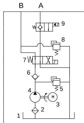
HYDRAULIC SCHEMATIC
