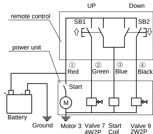
ELECTRICAL SCHEMATIC
