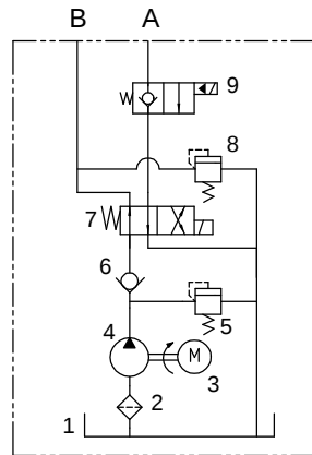
HYDRAULIC SCHEMATIC
