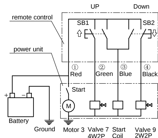
ELECTRICAL SCHEMATIC
