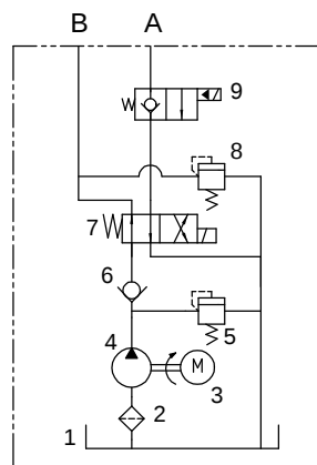
HYDRAULIC SCHEMATIC
