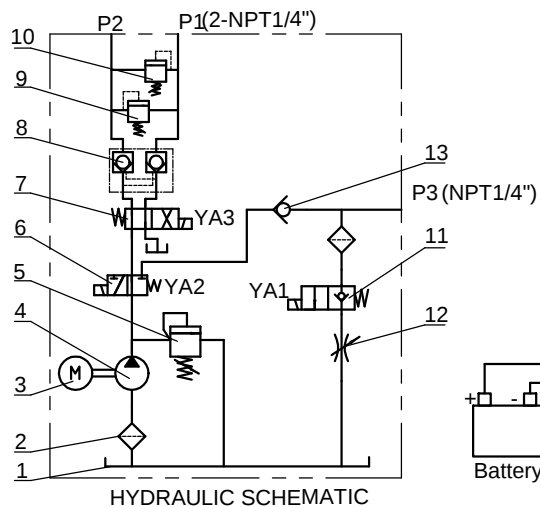
HYDRAULIC SCHEMATIC
