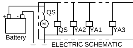
ELECTRIC SCHEMATIC
