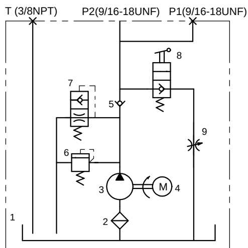
Hydraulic Schematic
