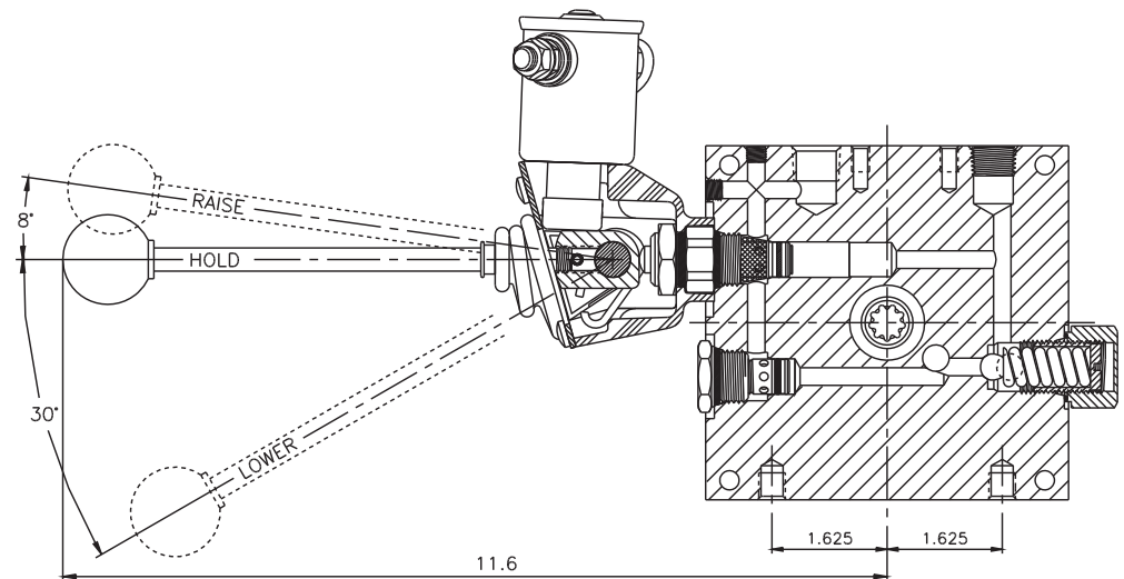
ENDHEAD SECTION
