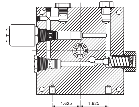
ENDHEAD SECTION
