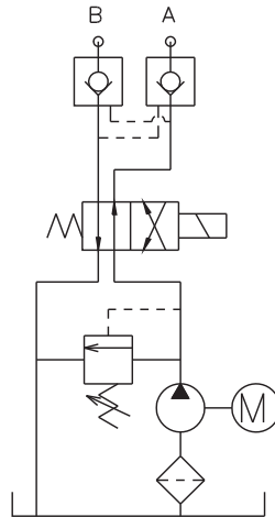
HYDRAULIC CIRCUIT
