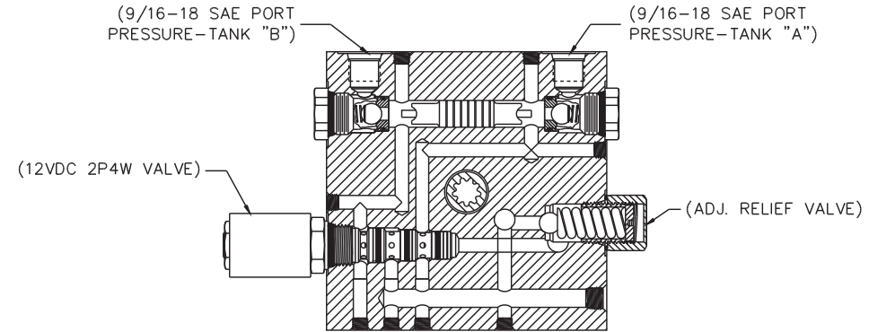
ENDHEAD SECTION
