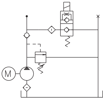
HYDRAULIC CIRCUIT
