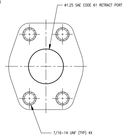
DETAIL B-B SCALE 1:1
