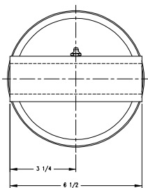
BUTT END VIEW HALF SCALE
