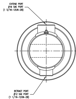
ROD END VIEW HALF SCALE
