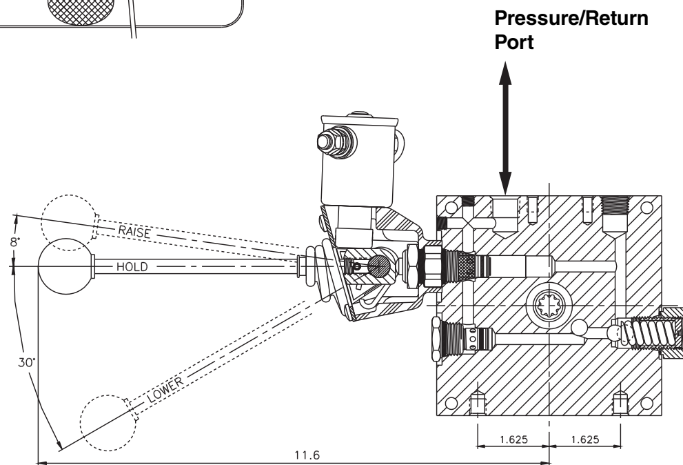
ENDHEAD SECTION
