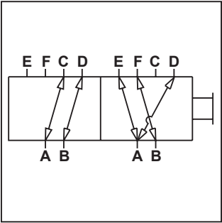
Circuit Diagram
